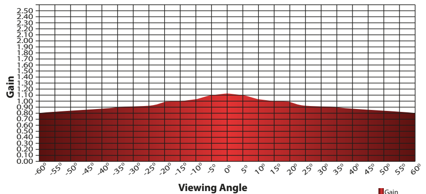
On axis 0° Gain: 1.1 | Viewing Cone: 180°
