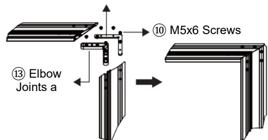
Corner connection
