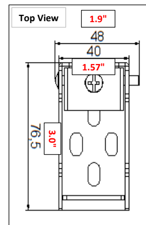
Wall/Ceiling Bracket Dims Unit of measure: mm / inch
